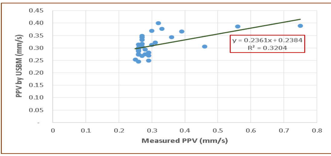
Figure 3.17. Measured and predicted PPV by USBM Equation
