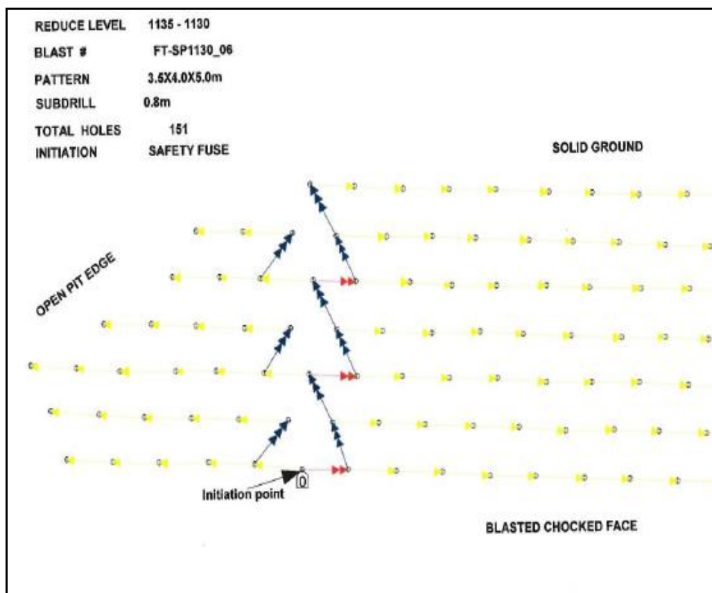
Figure 2.1. Blast design
