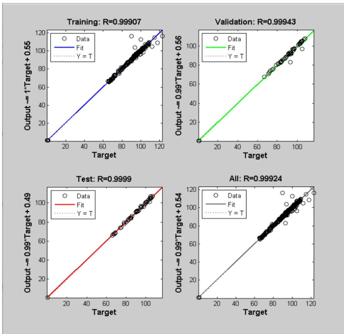
Neural network training regression plot for Tansig (eighteen neurons)
